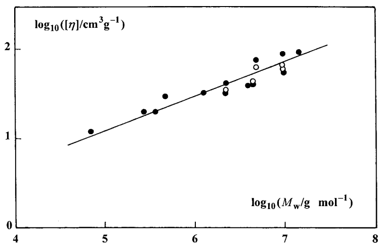
Fig. 2. \log_{10}[\eta] versus \log_{10}M_w (Mark-Houwink plot) for hydrolysed potato starches.
