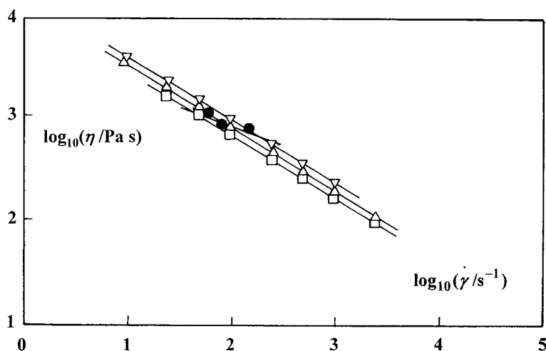
Fig. 4. Comparison of melt viscosities of a medium density polyethylene and a starch-water mixture. Polyethylene: \square 230°C, \Delta 210°C, \nabla 190°C. Starch-water, 17% water, \bullet 175°C (metering zone); apparent melt viscosities from back-pressure experiments using a standard Arbarg injection moulding machine.
