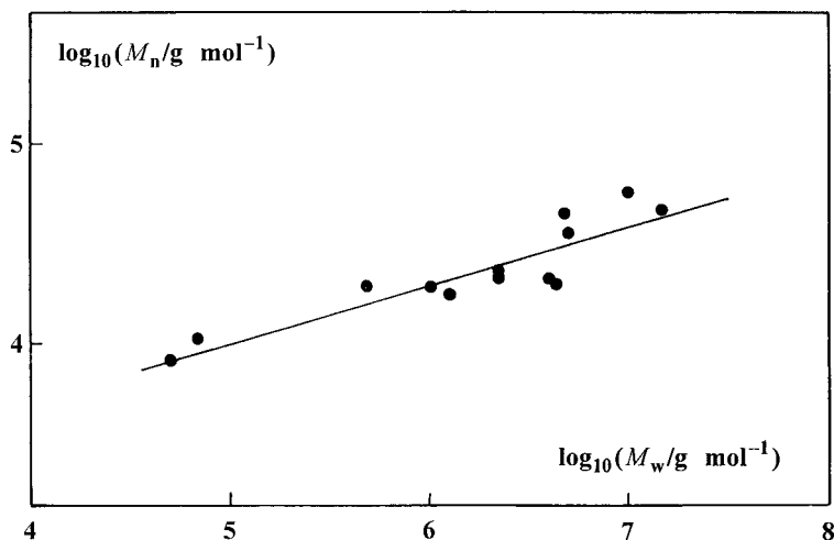
Fig. 3. \log_{10}M_n versus \log_{10}M_w for hydrolysed potato starches. Least-squares line gives M_n/\text{g mol}^{-1} = 405(M_w/\text{g mol}^{-1})^{0.28} .
